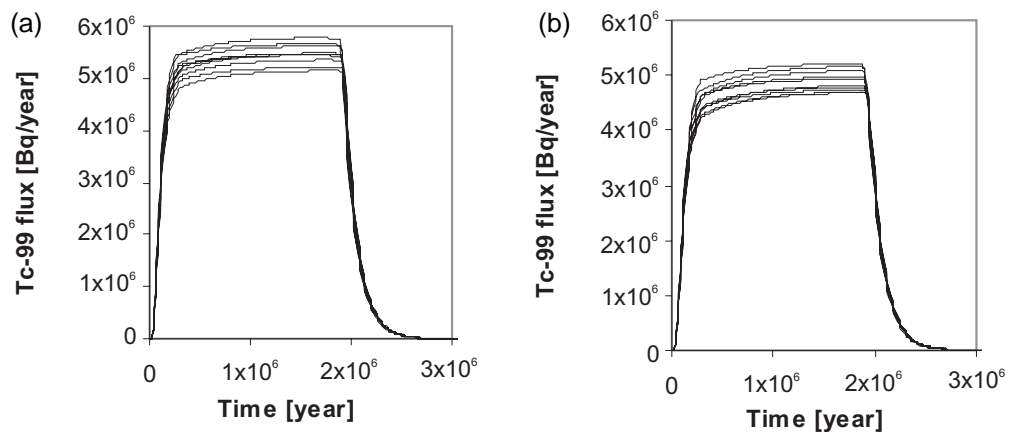
Fig. 1 Total 99 Tc fluxes for ten different simulations through (a) the lower clay-aquifer interface and (b) the upper clay-aquifer interface.
