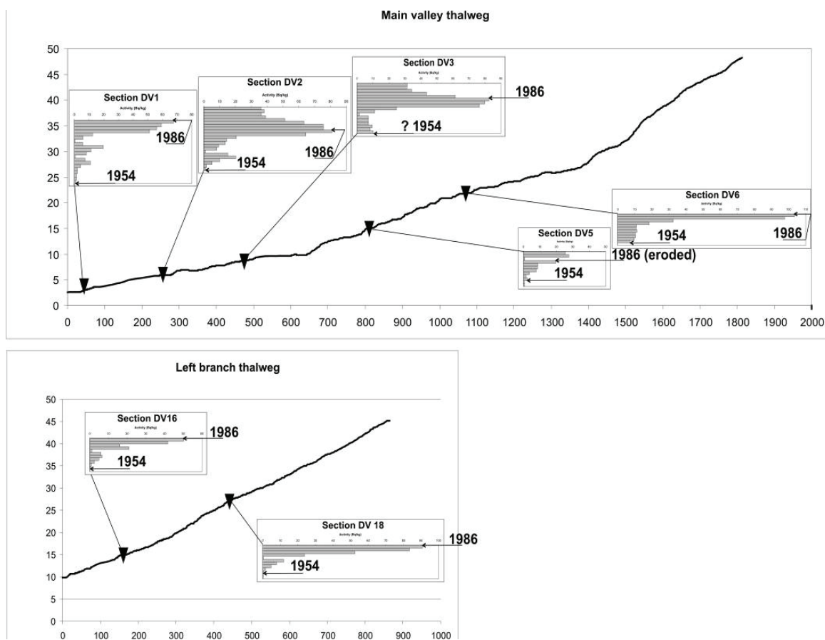
Fig. 3 Longitudinal profiles of the main valley and the right tributary hollow (upper graph) and of the left tributary hollow (lower graph) with vertical distribution of ^{137}\text{Cs} (scale exaggerated) in sampled sections (designated by black triangles).
