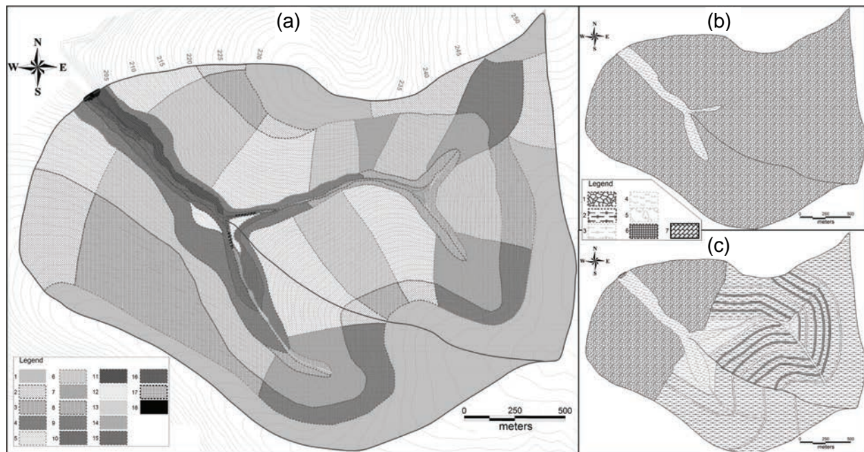
Fig. 2 (a) Geomorphic map of the case study catchment (topography contours are drawn in 1 m intervals). Legend: (1) Rolling interfluvial surfaces with dominant gradients <2^\circ ; (2–4) Gradual slopes, 2\text{--}3^\circ (2), divergent; (3), straight; (4), convergent; (5–7), moderate slopes, 3\text{--}5^\circ (5, divergent; 6, straight; 7, convergent); (8), moderately sloping sides of tributary hollows, 3\text{--}5^\circ ; (9), relatively steep slopes and sides of tributary hollows, 5\text{--}10^\circ ; (10), moderately sloping main valley sides, 5\text{--}10^\circ ; (11), relatively steep main valley sides, >10^\circ ; (12), main valley terrace surfaces, 2\text{--}5^\circ ; (13), bottoms of slope depressions; (14), bottoms of tributary hollows; (15), main valley bottom; (16), aggraded reservoir bottom; (17), concrete troughs at sites of former gauging stations at outlets of tributary hollows; (18), earthen dam. (b) Land use before 1986. (c) Land use after 1986. Legend: (1), traditional cultivation; (2), soil-protective cultivation; (3), soil-protective cultivation parcels left under perennial grasses; (4), pasture and hay-mowing lands in valley bottoms and along grass-covered waterways; (5), forest shelter belts; (6), contour terraces; (7), earthen dam.
