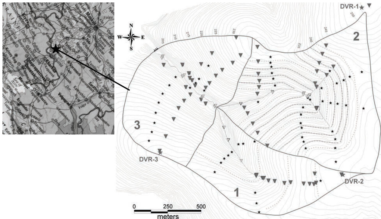
Fig. 1 Approximate location of the study catchment within the Russian Plain and location of sampling points within the Gracheva Loschina catchment. Legend: (1) DVR-1–DVR-3 and larger stars designate reference point locations (DVR-4 is located outside the map, about 1 km to the northwest of the study catchment); (2) grey triangles designate soil survey sections in the bottoms of the main valley and its two upper branches; (3) black triangles designate soil survey sections along slope transects; (4) smaller stars designate ^{137}\text{Cs} integral sampling points along slope transects; (5) dotted lines designate forest shelter belts; (6) hatched lines designate contour terraces; and (7) large digits designate subcatchment numbers as referred to in the text below. Topography contours are drawn at 1 m intervals.
