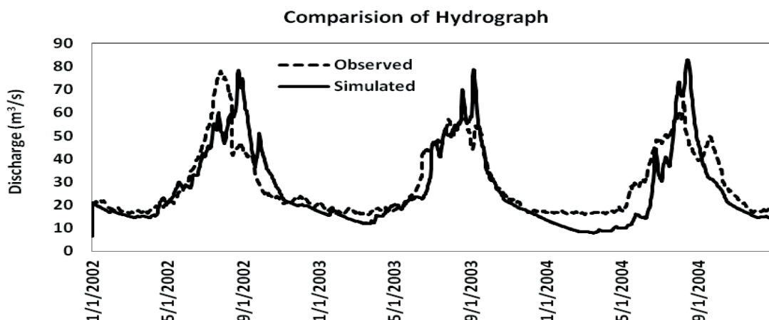
Fig. 2 Discharge calibrated hydrograph of Langtang Khola.
