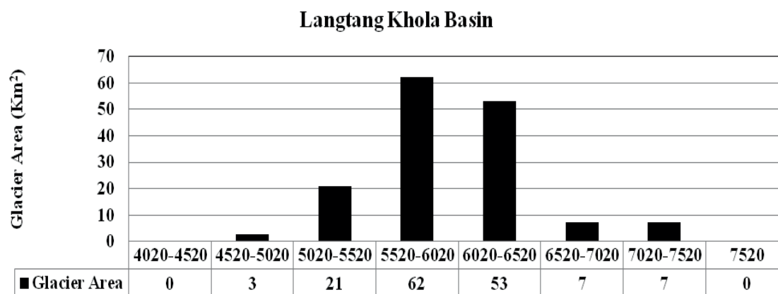
Fig. 2 Glacier Area in elevation wise.
