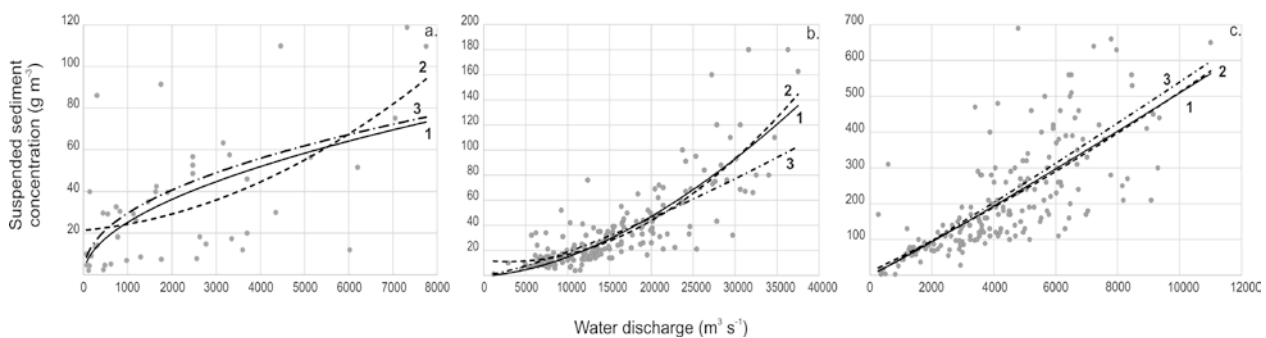
Fig. 4 Sediment rating curves for the Anabar River at (a) Saskylakh, (b) the Lena River at Tabaga and (c) the Indigirka River at Vorontsovo, obtained using non-linear power fit (1), non-linear power fit with additive constant (2) and log-linear fit (3).
