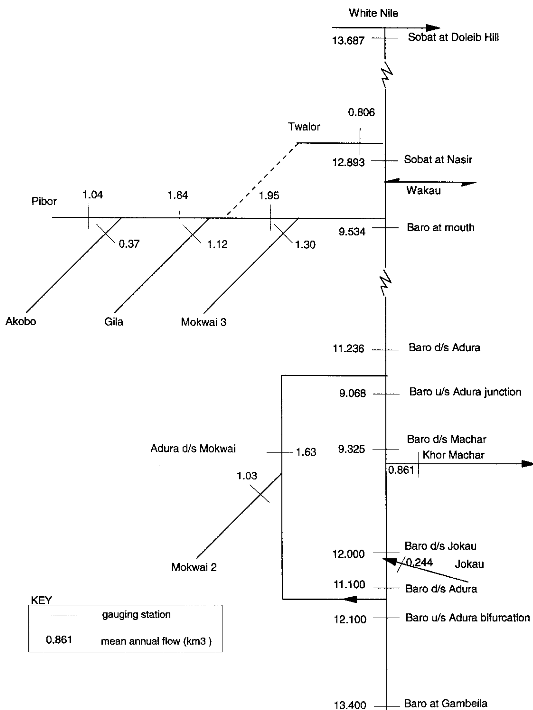
Fig. 7.5 Schematic plan of Baro-Pibor basins and mean annual flows, km 3 .
