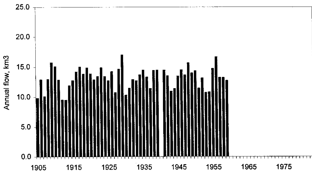
Fig. 7.2 Baro at Gambia: annual flows, 1905–1959.
