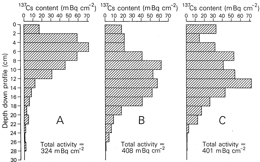
FIG. 2 Typical examples of the vertical distribution of ^{137}\text{Cs} in soil profiles associated with undisturbed permanent pasture (A) and arable cultivation (B).
