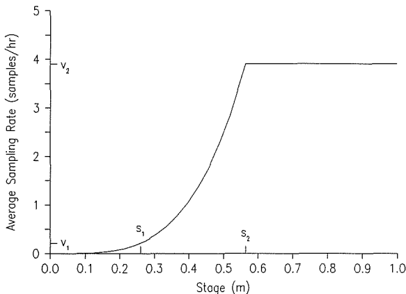
Fig. 1 A typical ASR (Average Sampling Rate) curve for the PSALT (Piecewise Selection At List Time) technique. The lower and upper design stages are s_1 and s_2 with associated design average sampling rates of v_1 and v_2 . The ASR is constant at v_2 for stages above s_2
