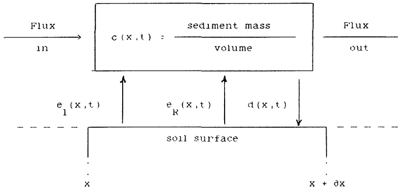
Fig. 1 Definition sketch of overland flow erosion/deposition system.
