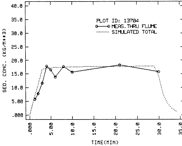
Fig 3 Sedigraph for very wet run on bare plot.
