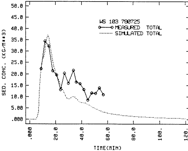
Fig. 4 Sedigraph for the storm event of 07/25/78 on WS 103.
