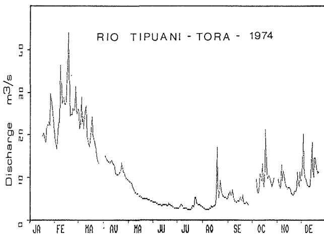
Fig. 3 Discharge hydrography of the River Tipuani at Tora, 1974 (from SENAMHI).
