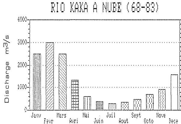
Fig. 2 Hydrological regime of the River Kaka at Nube, 1968-1983 (from SENAMHI).
