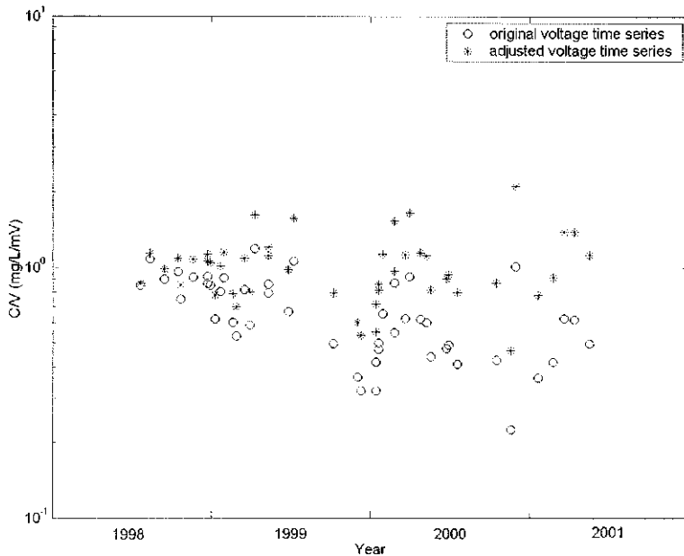
Fig. 1 Ratio of suspended-sediment concentration to sensor voltage ( C/V ) as a function of time in the Sacramento River at Freeport, California. Drift of the sensor is indicated by the decrease in C/V with time for the original voltage time series. The adjusted voltage time series did not drift with time.
