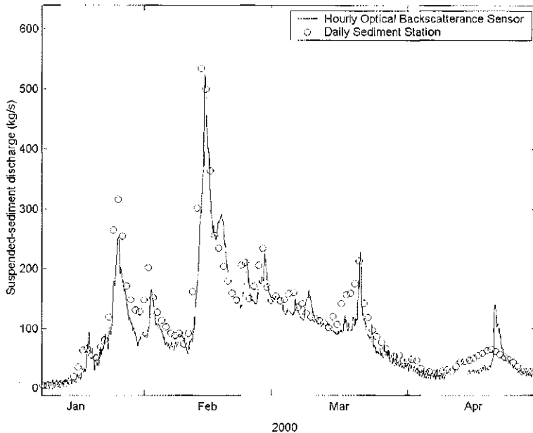
Fig. 5 Suspended-sediment discharge in the Sacramento River at Freeport, California, January–April 2000. Sediment station data are from Anderson et al. (2001).
