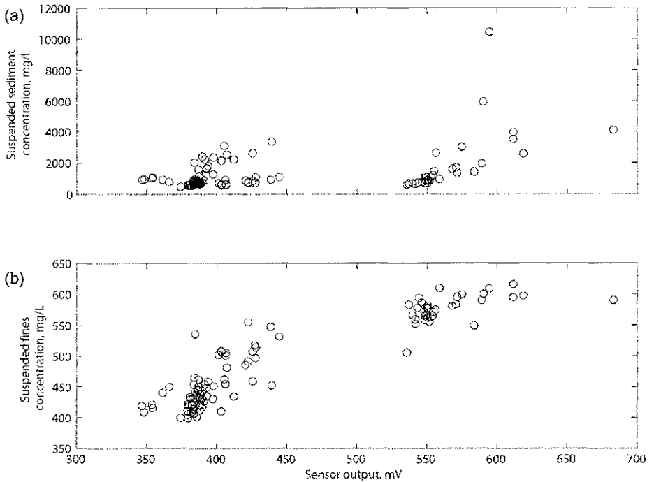
Fig. 4 Calibration of an optical backscatterance sensor in the Colorado River at Cisco, Utah. Sensor output correlates poorly with suspended sediment concentration (a), but correlates well with the suspended fine sediment concentration (b). Five data points with large concentration or sensor output are not included for clarity.
