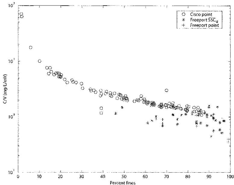
Fig. 3 Ratio of suspended-sediment concentration to sensor voltage ( C/V ) as a function of the fraction of fine sediment in the Sacramento River at Freeport, California, and in the Colorado River at Cisco, Utah. C/V for any data point is approximately equal to the slope of a calibration line through that point. A different sensor was used at each site and each sensor has slightly different optical characteristics, so the difference in the trend of C/V , not the absolute value of C/V , should be compared between the sites.
