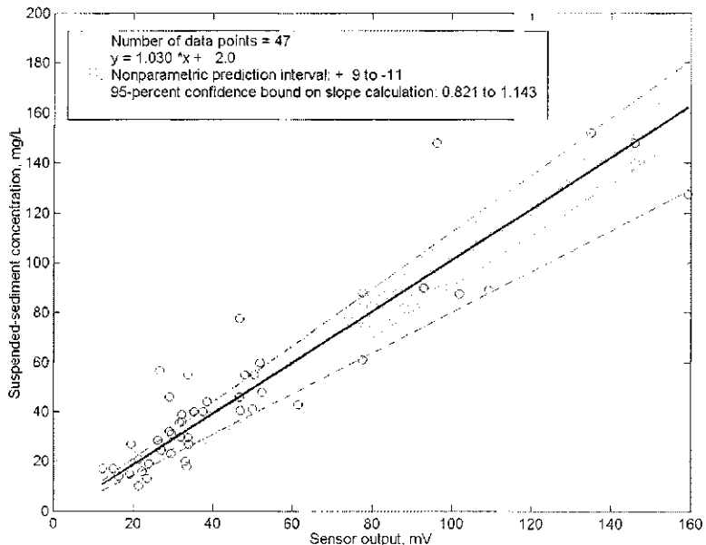
Fig. 2 Calibration of an optical backscatterance sensor in the Sacramento River at Freeport, California. Sensor output drift has been corrected.
